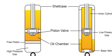
BILSTEIN'S MONOTUBE vs. COMPETITOR'S DUALTUBE
